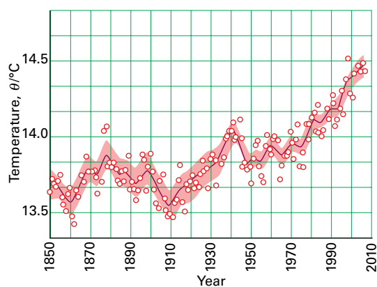
Fig. 2 The average change in surface temperature of the Earth from 1850 to 2010.
