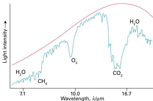
Fig. 1 The intensity of infrared radiation that would be lost from Earth in the absence of greenhouse gases is shown by the red line. The blue line is the intensity of the radiation actually emitted. The maximum wavelength of radiation absorbed by each greenhouse gas is indicated.
